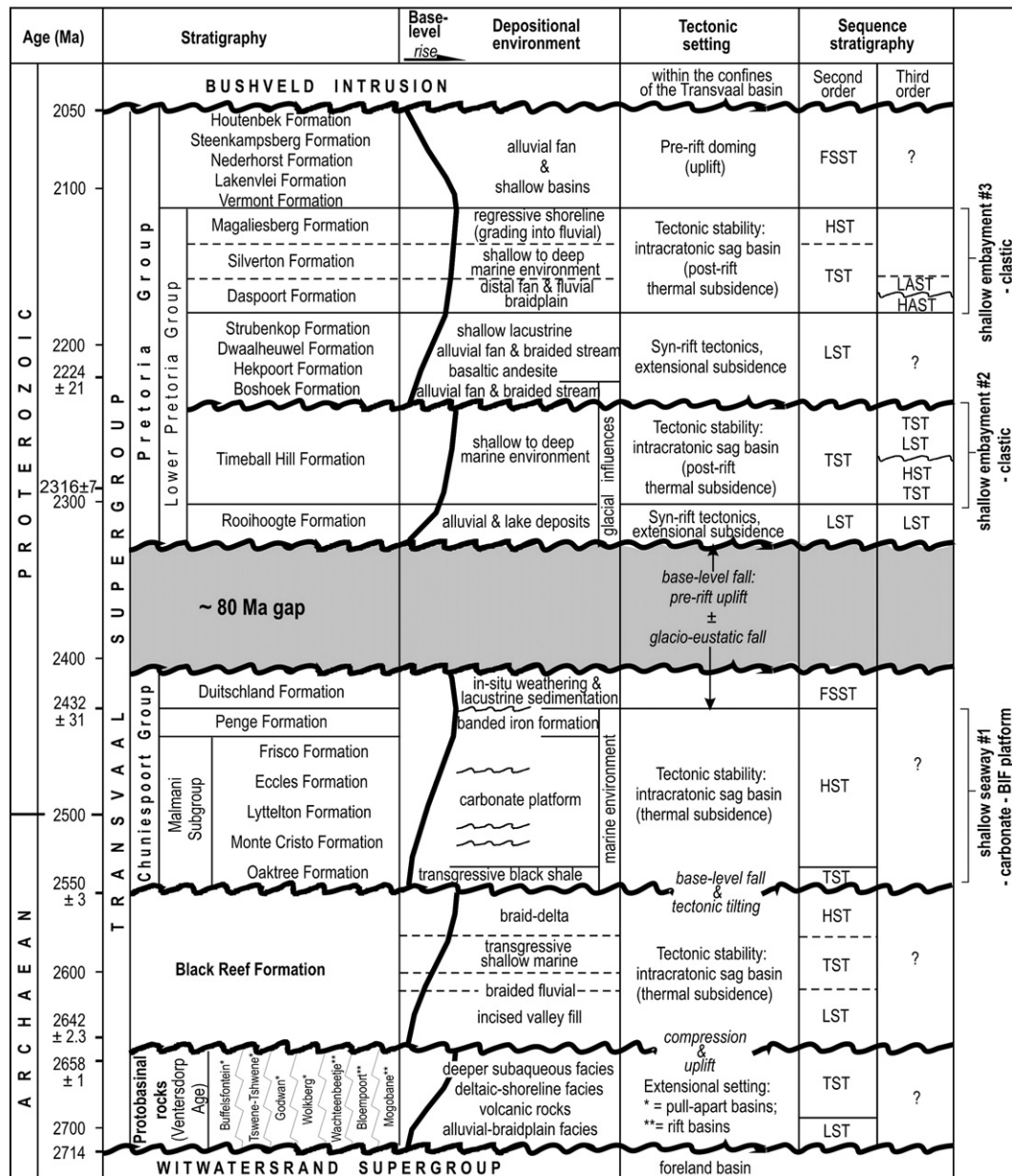
Fig. 2. Schematic geodynamic history chart proposed for the Transvaal Supergroup (first-order sequence) in the Transvaal basin: summarizes lithostratigraphy, chronology, inferred depositional paleoenvironments and tectonic settings, as well as interpreted second- and third-order sequence stratigraphy (modified after Catuneanu and Eriksson, 1999; Eriksson et al., 2001). Age near base of Pretoria Group (lower Timeball Hill Formation) is from Hannah et al. (2004) with remaining age data from references in Eriksson et al. (2001). Note the Daspoort and Magaliesberg Formations, discussed in this paper, near the top of the uppermost Pretoria Group, in the middle of the youngest second-order sequence, concomitant with the base-level maximum.
