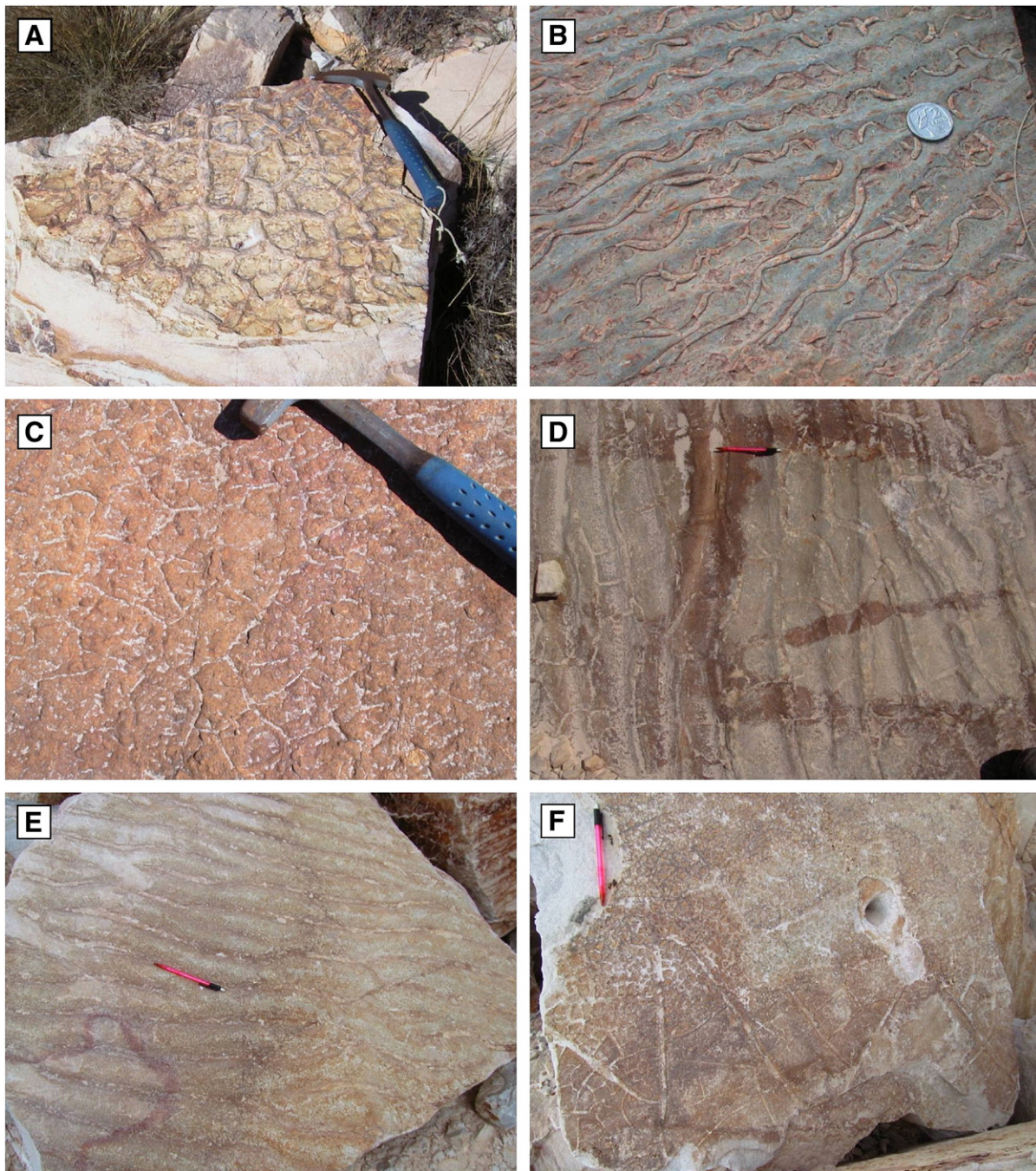
Fig. 6. Mat-related structures (MRS) from the Magaliesberg Formation collected from two study sites and typical of the MRS to be found associated with the ripple fields (Fig. 5) at most outcrops. (A) Polygonal petee ridges, showing two orders; (B) Manchuriophycus , sinuous sand cracks formed within ripple troughs (photo: Pieter Bosch); (C) reticulate crack pattern of “elephant skin texture”, preserved as negative features on the sole of a sandstone bed; (D) ripple crest sand cracks; note secondary cracks cutting across ripple troughs, and main crack bifurcation; (E) sand cracks, localized within ripple troughs; in contrast to those shown in B ( Manchuriophycus ), these cracks are relatively straight and approximately parallel to ripple crests; and (F) wrinkle structures (top left part of block near pen) passing into wedge-shaped petee ridges (bottom right of drilled quarry block). Modified from Eriksson et al. (2010).
