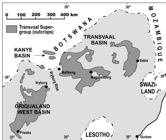
Fig. 1. Sketch map showing the three preservational sub-basins of the Transvaal Supergroup: Transvaal itself, separated from the Griqualand West sub-basin by the Vryburg Rise paleohigh, and the Kanye sub-basin in Botswana, north of the paleohigh.
