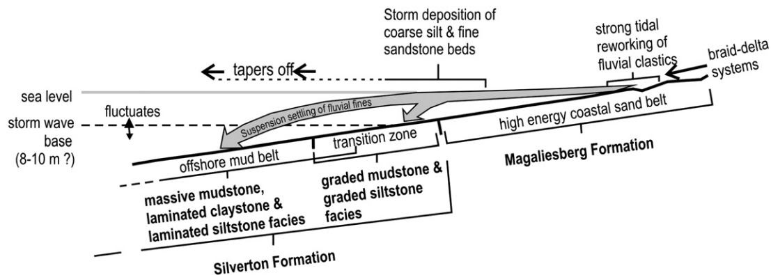
Fig. 4. Schematic sketch of paleoenvironmental model postulated for the fine-clastic epeiric sea interpreted for the Silverton Formation, and its sandy coastal zone interpreted for the Magaliesberg Formation. Modified after Eriksson et al. (2008).
