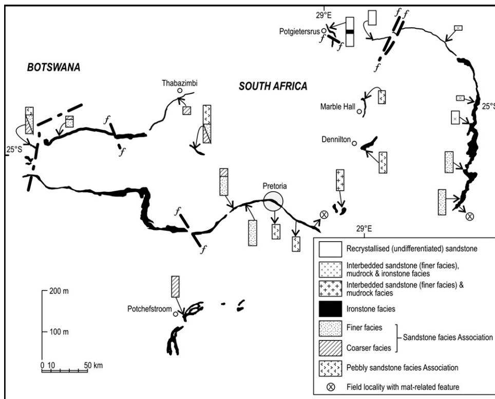
Fig. 3. Schematic illustration of vertical and lateral arrangements of facies/facies associations, as identified at field sites across the preserved Daspoort basin (modified from Eriksson et al., 1993; Eriksson and Catuneanu, 2004). Note two field localities indicated, where mat-related features were found.
